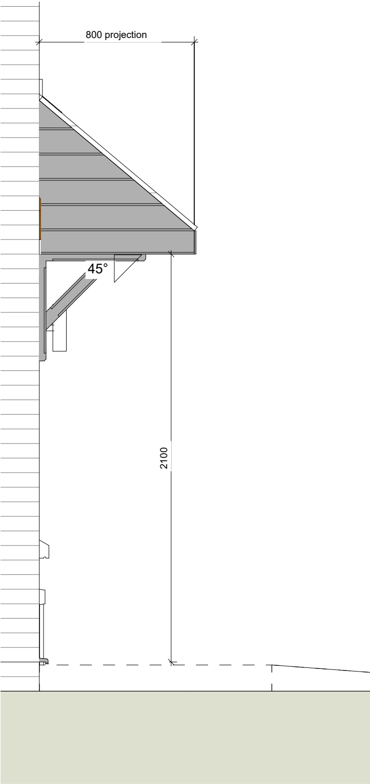
1 Gable Elevation 1 : 20
