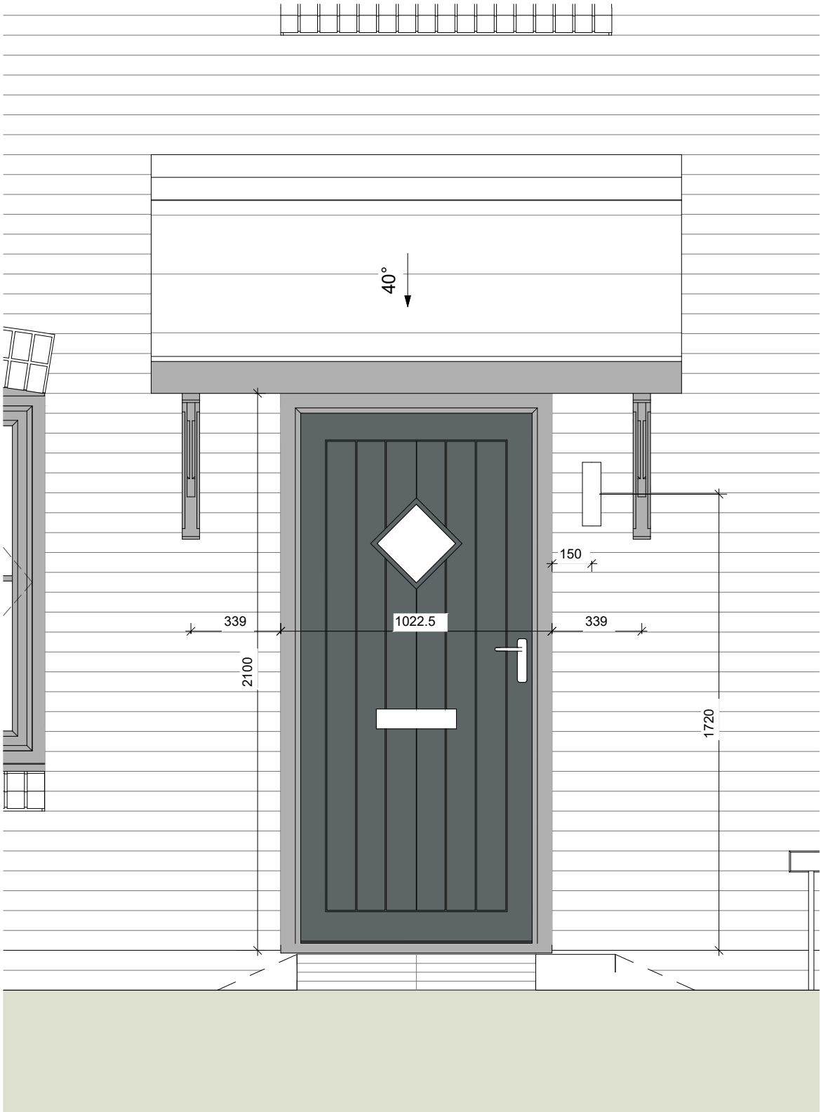
2 Front Elevation 1 : 20
